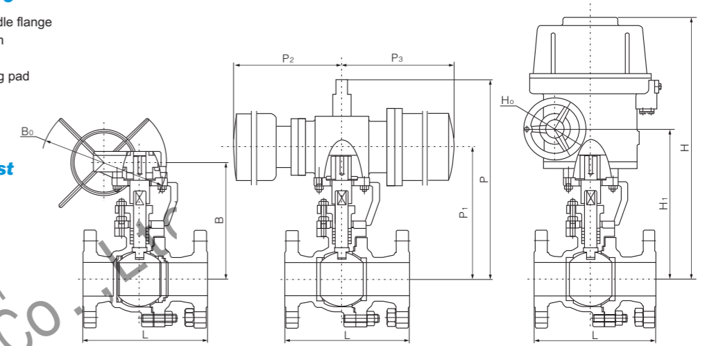
Main size of outside & weight
