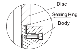
Elastic Ring Hard Seal Structure
