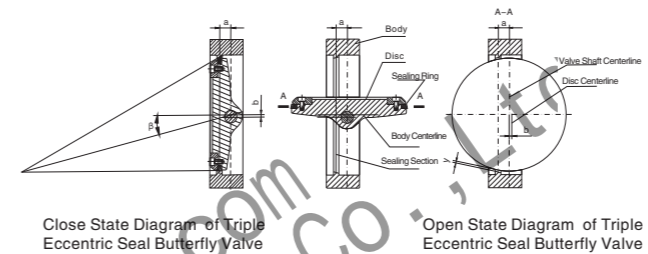
Sealing Principle of Triple Eccentric Seal Butterfly Valve
