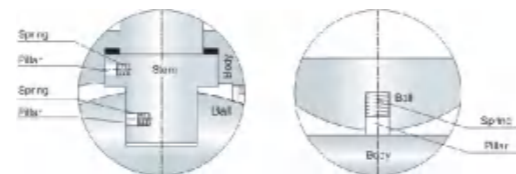
Anti-Static design for ball valve ∅32mm Anti-Static design for ball valve ∅25mm
