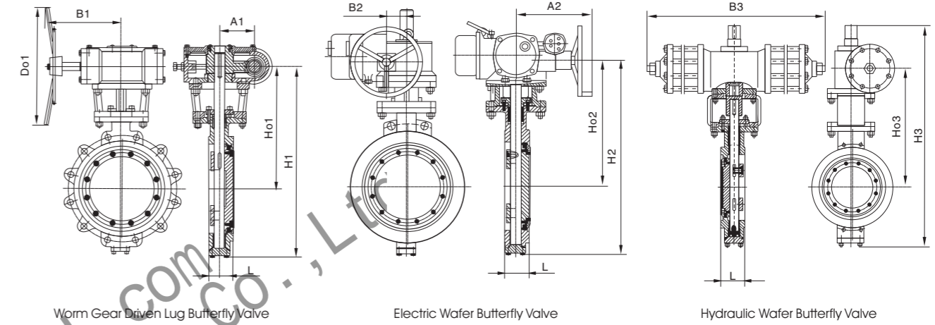
Main size of Wafer Butterfly Valve outside & weight
