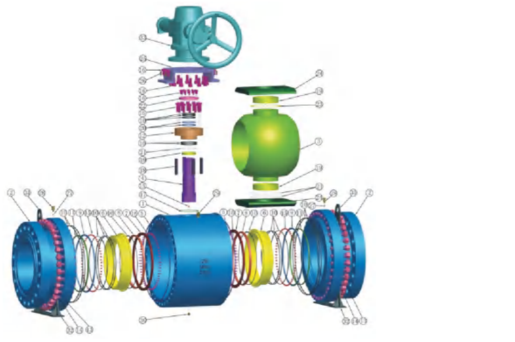
ASTM Material list of cast steel trunnion mounted ball valve
